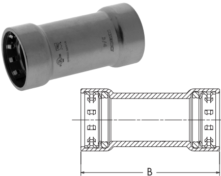
PC201 (No Stop) Repair Coupling P x P – Carbon Steel
