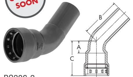
PC206-2 45° Elbow Ftg x P – Carbon Steel
