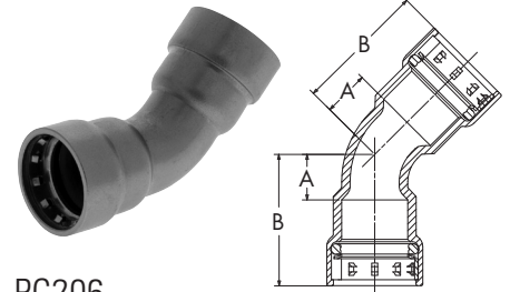
PC206 45° Elbow P x P – Carbon Steel
