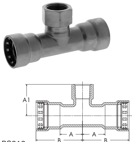
PC212 Tee P x P x F – Carbon Steel
