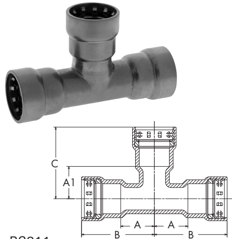
PC211 Tee P x P x P – Carbon Steel
