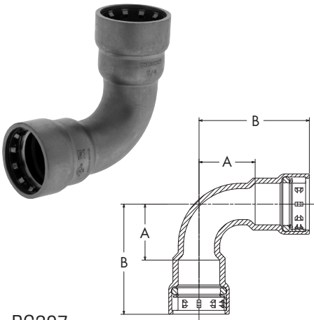
PC207 90° Elbow P x P – Carbon Steel
